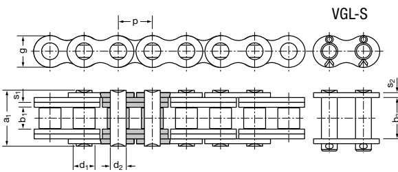
Plate link chain RLK 50-1 SL/A, Plate link chain 64-1 S / SH / SH
