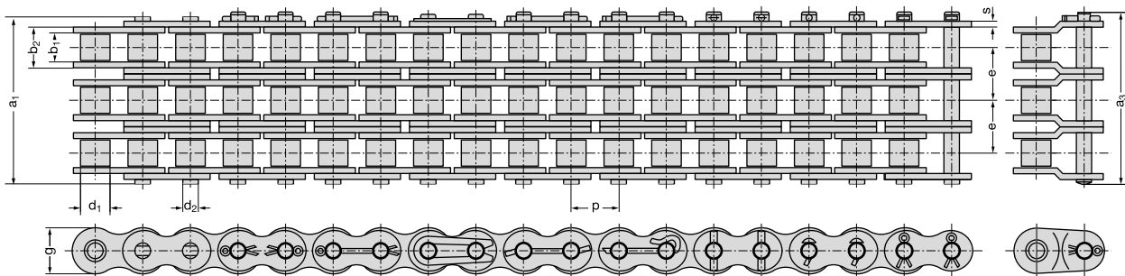
B Inner link A Outer link AS Outer link AT Outer link H Connecting link with shepherd crook cotter AK Outer link U Outer link with cotter L Cranked link with cotter
