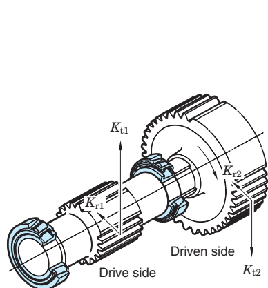
Fig. 5-1 Load on spur gears
