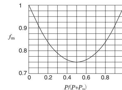
Fig. 5-6 Coefficient f_m
