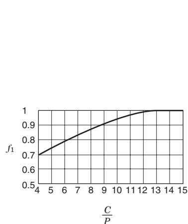
Fig. 8-1 Values of correction coefficient f_1 of load magnitude
